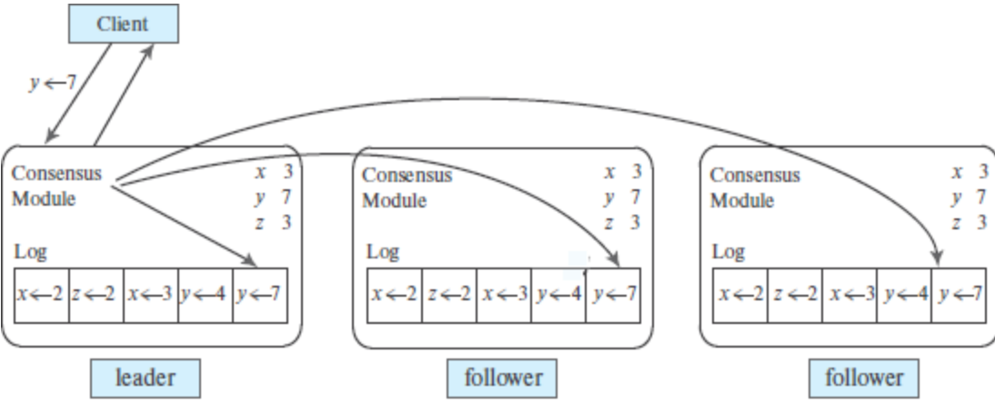
Leader declares log record committed after it is replicated at a majority of nodes. Update of state machine at each replica happens only after log record has been committed.
