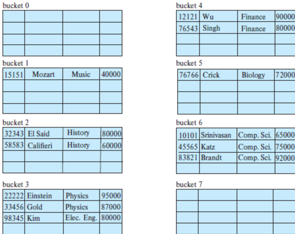
Figure 24.7 Hash organization of instructor file, with dept_name as the key.
