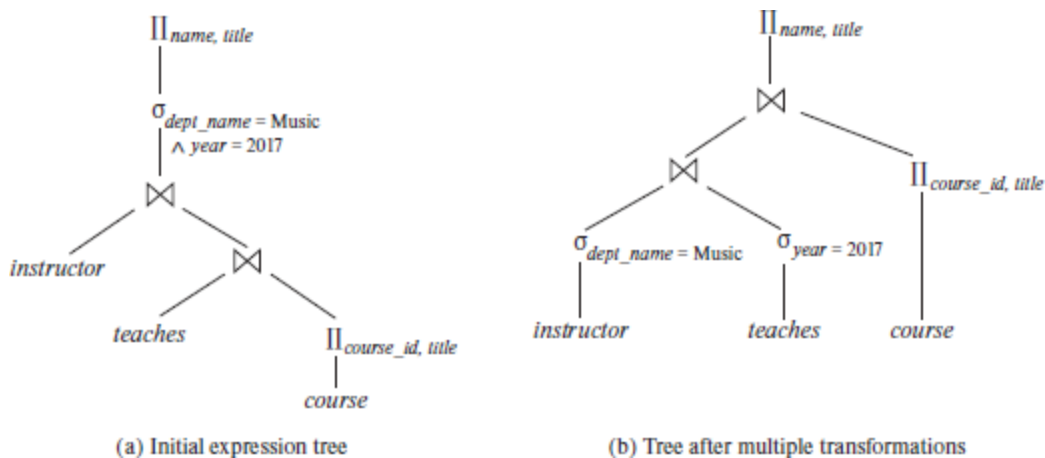
Figure 16.4 Multiple transformations.
