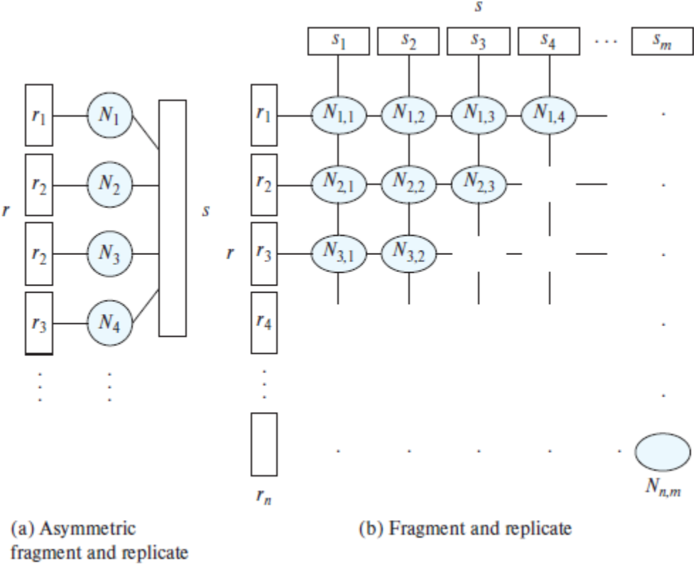
Figure 22.3 Fragment-and-replicate schemes.
