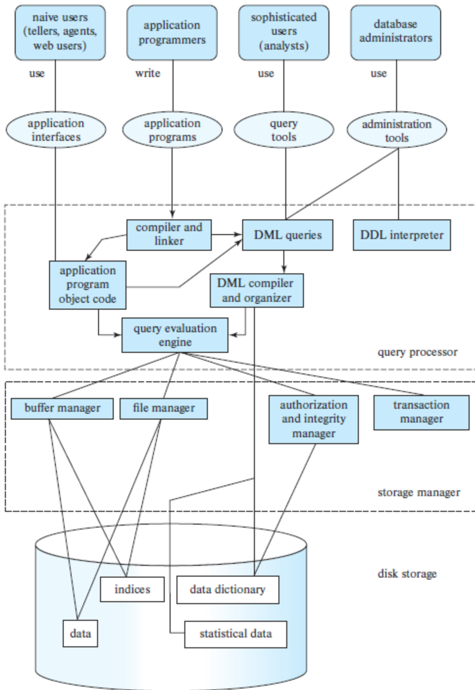
Figure 1.3 System structure.
