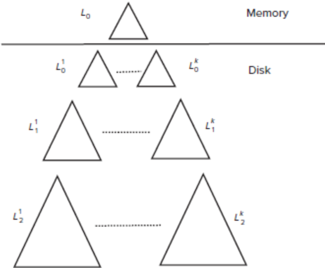
Figure 24.2 stepped-merge index
