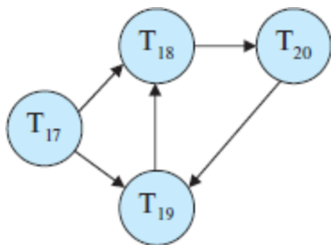
Figure 18.14 Wait-for graph with a cycle.
