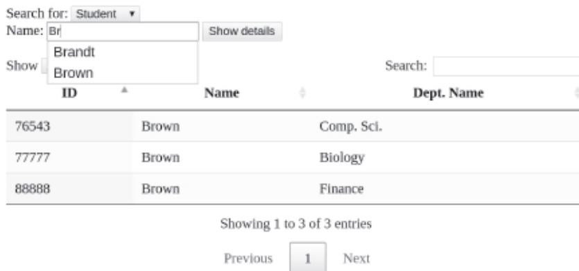
Figure 9.13 Screenshot of display generated by Figure 9.12 .
