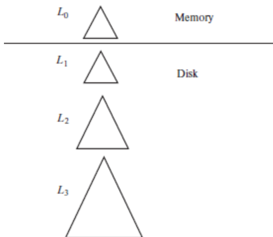
Figure 24.1 Log-structured merge tree with three levels.
