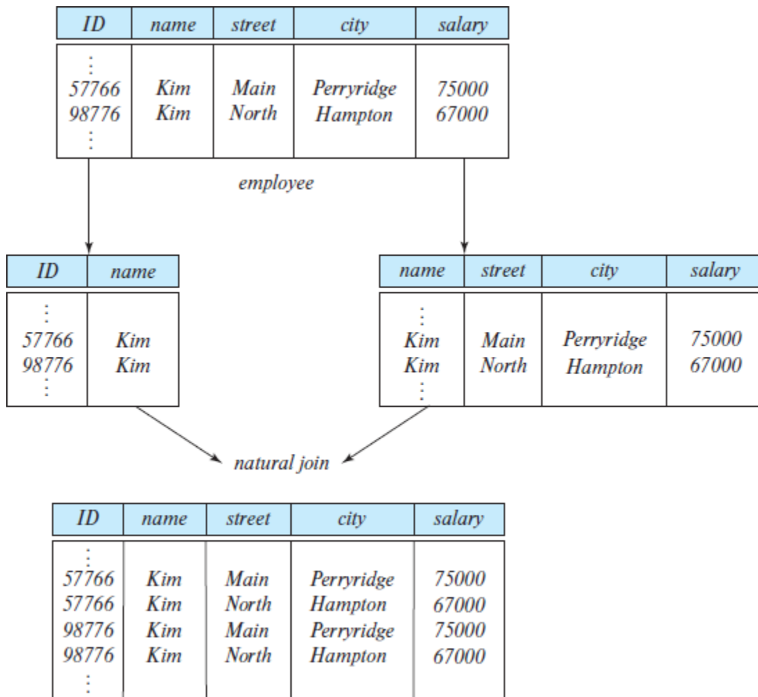
Figure 7.3 Loss of information via a bad decomposition.
