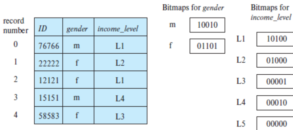
Figure 14.28 Bitmap indices on relation instructor_info .
