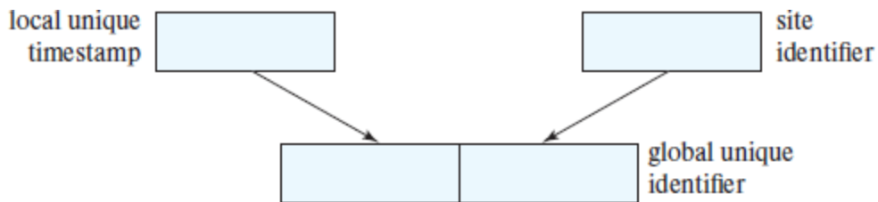
Figure 23.7 Generation of unique timestamps.
