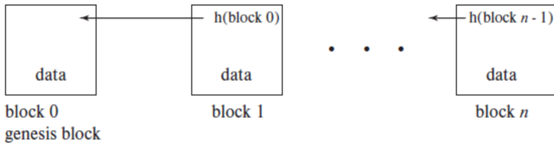
Figure 26.1 Blockchain data structure.
