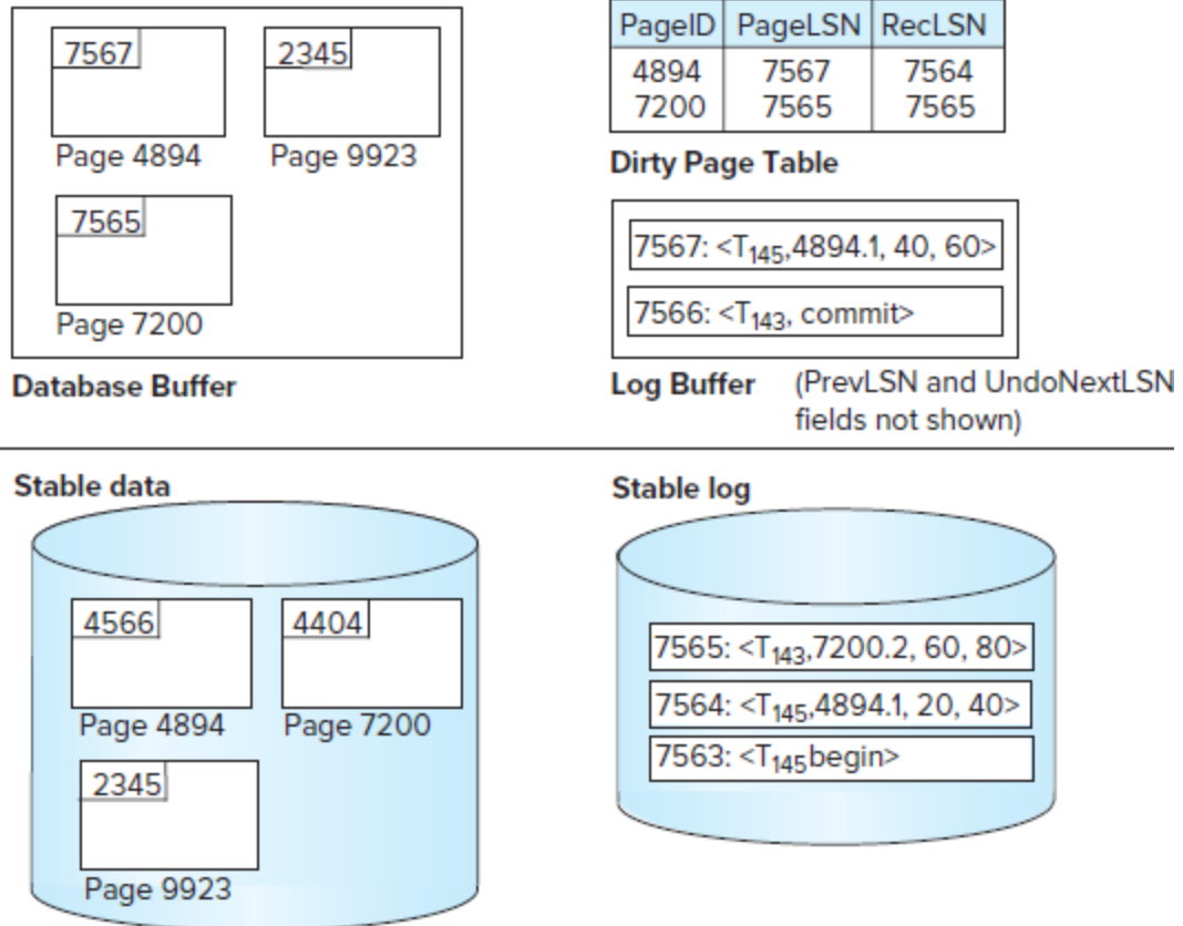
Figure 19.9 Data structures used in ARIES.
