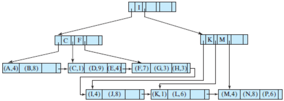
Figure 14.22 B + -tree file organization.
