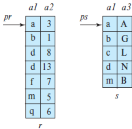
Figure 15.8 Sorted relations for merge join.
