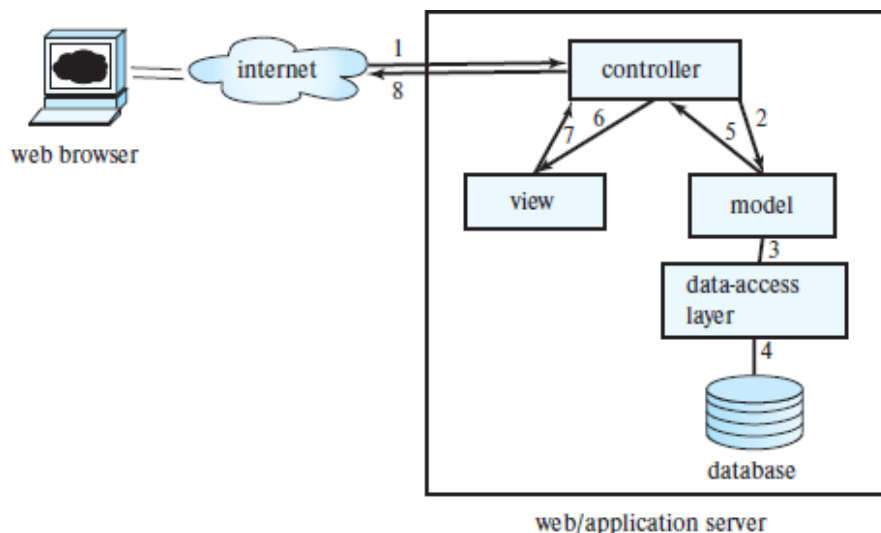
Figure 9.14 Web application architecture.
