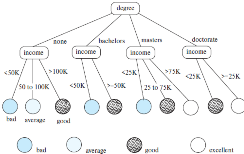
Figure 11.11 Classification tree.
