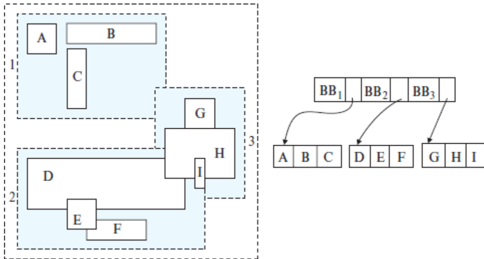
Figure 24.5 An R-tree.
