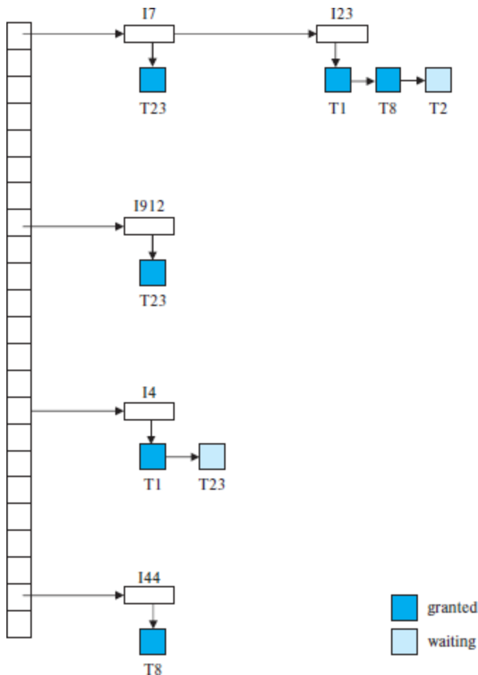
Figure 18.10 Lock table.
