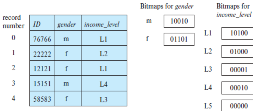
Figure 24.3 Bitmap indices on relation instructor_info .
