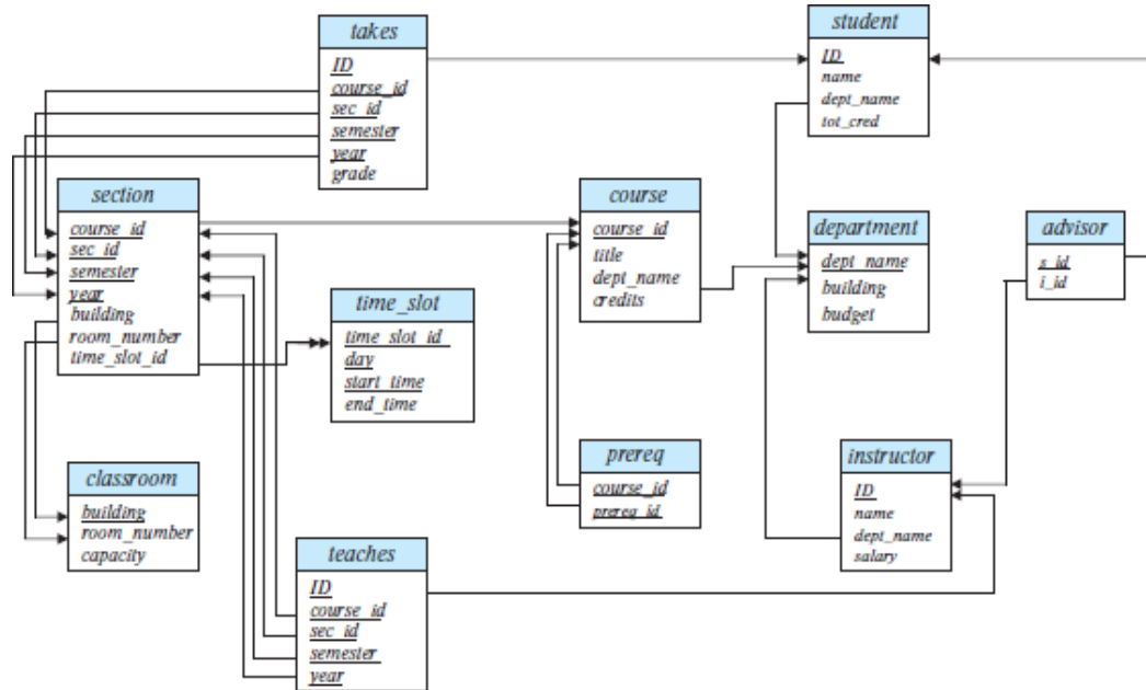
Figure 2.9 Schema diagram for the university database.
